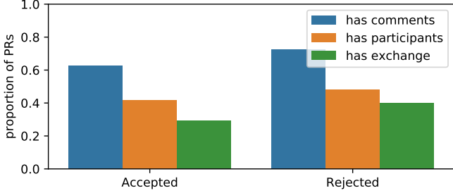
Fig. 2. Proportion of accepted and rejected PRs w.r.t. the presence of comments and participants.
