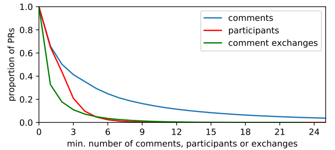
Fig. 1. Proportion of PRs having at least a given number of comments, participants or comment exchanges.
