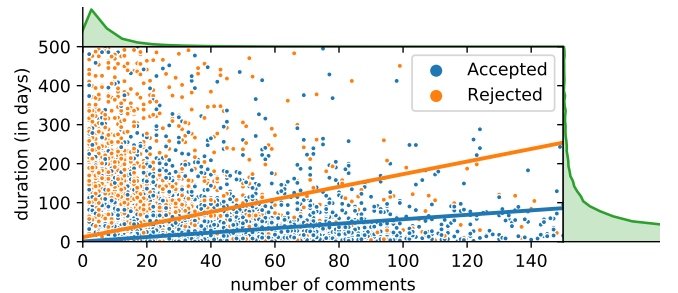
Fig. 5. Scatter plot and density plots of discussion duration and number of comments.
